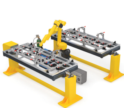
■ Single Axis Head & Tail Positioner
